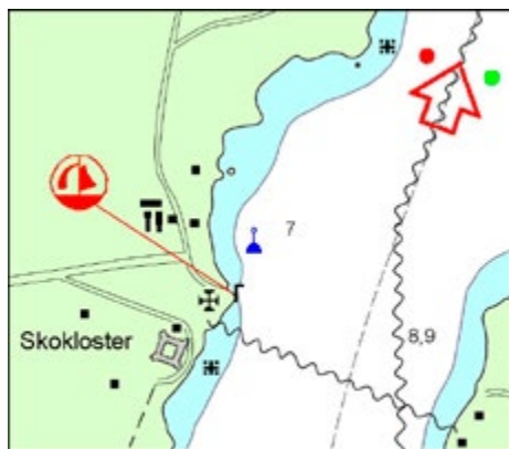
Skokloster N 59°42',360 E 17° 37',566
